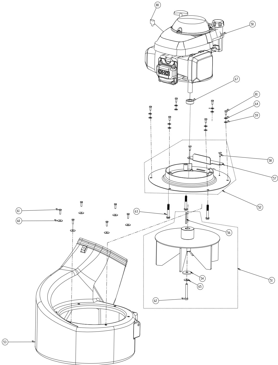
Engine Assembly
